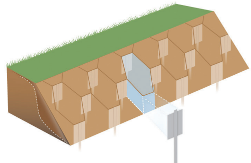
Geopier Plate Pile™ elements form a series of horizontal barriers where the soil arches between the plates.
